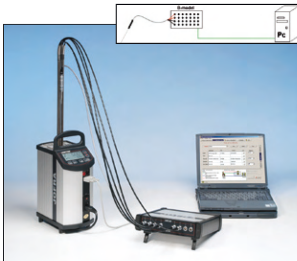
Picture 2: ASM-803 B performing its own measurements in a JOFRA ITC-320 A including an STS reference sensor in channel one all controlled by JOFRACAL.
