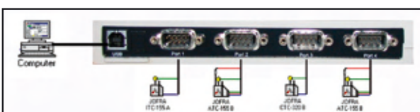
Edgeport converter - Order number 125002 The edgeport converter converts one USB port to four RS232 ports without external power supply. Tested with JOFRA calibrators and JOFRACAL calibration software
